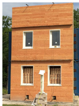
Lepir 2 test - France.
