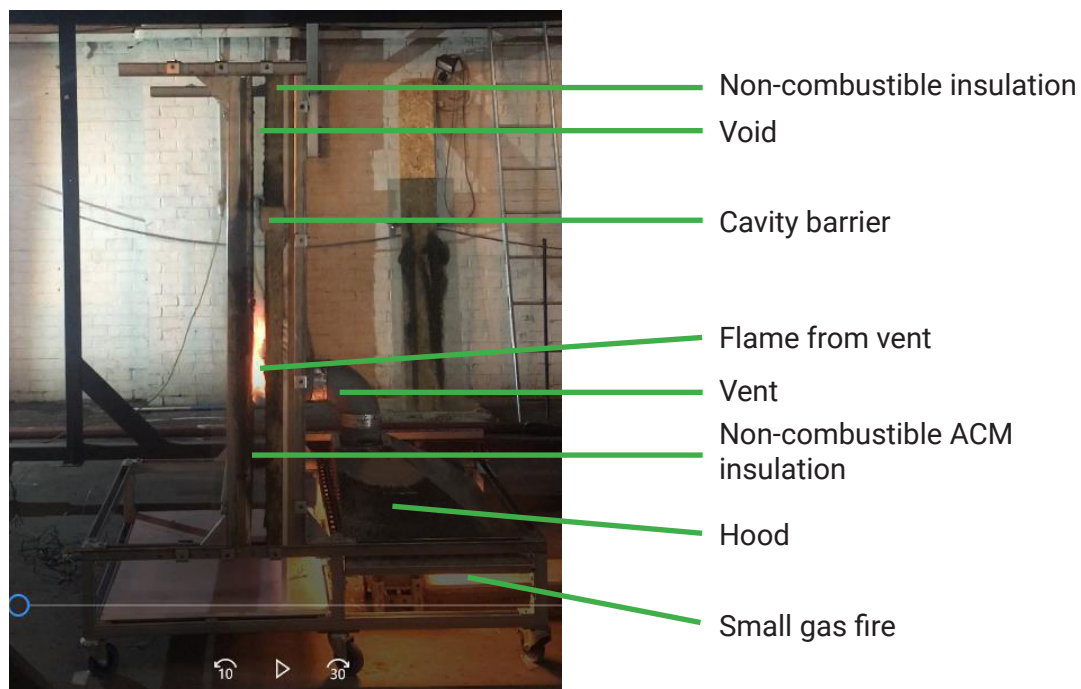
Figure 34 - Cavity barrier test rig
